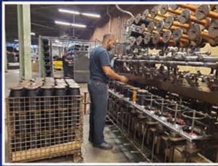
The yarn is twisted into 3-Strand twine.
